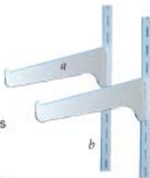
a. Bracket - 16 gauge steel, assorted sizes and finishes b. Standard - 5/8" wide, adjustable on 1" centers, various lengths 16 gauge steel
